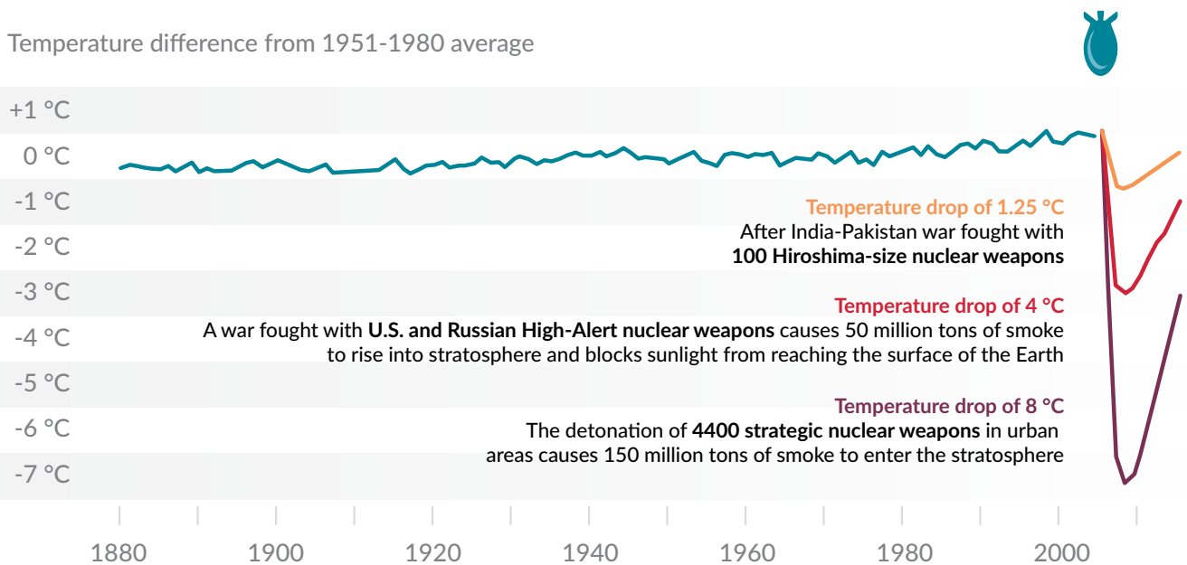
Figure 8: Global average surface temperature changes estimated in cases of small, moderate and large nuclear wars in the context of the change of climate since 1880 (Source: nucleardarkness.org)
